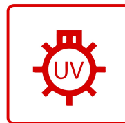
Polymerization
